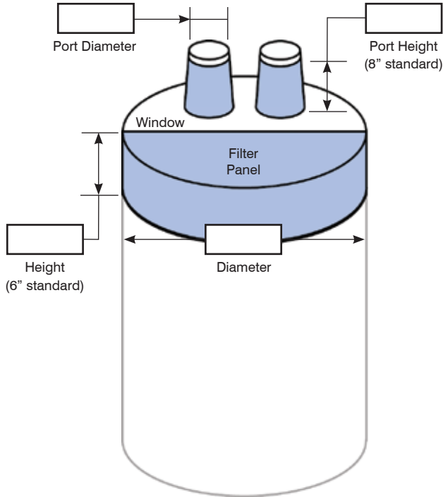
DP Style (Featuring Two Ports)
